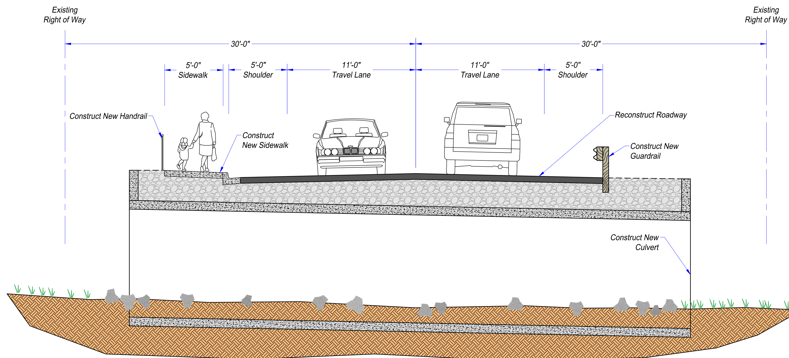
CULVERT SECTION Not To Scale
