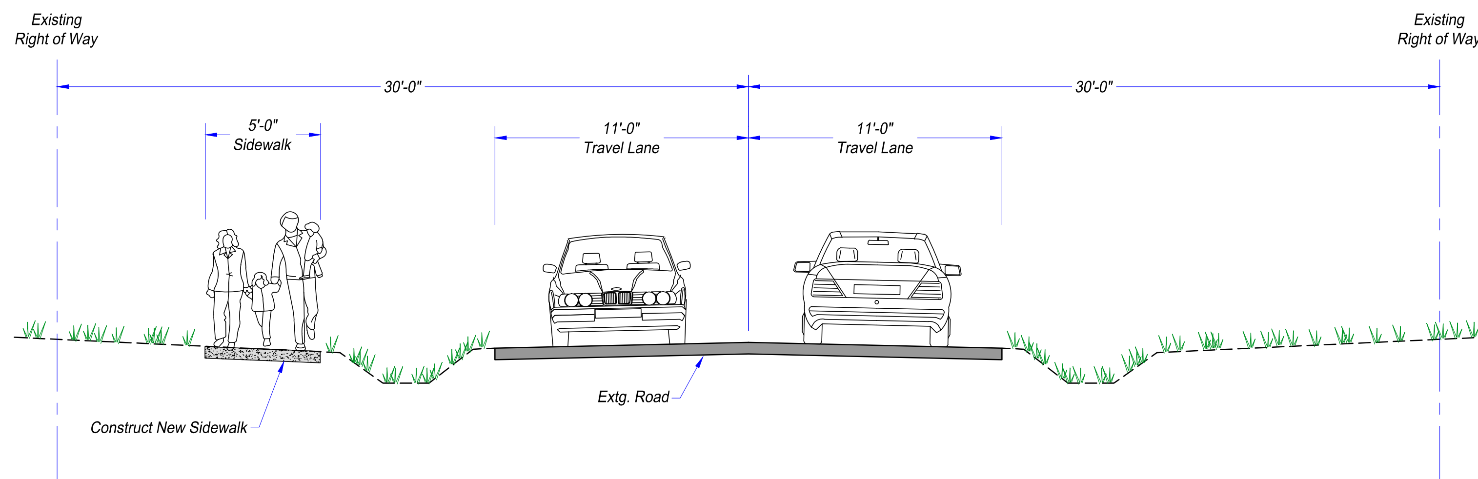
SEPARATED SIDEWALK SECTION Not To Scale
