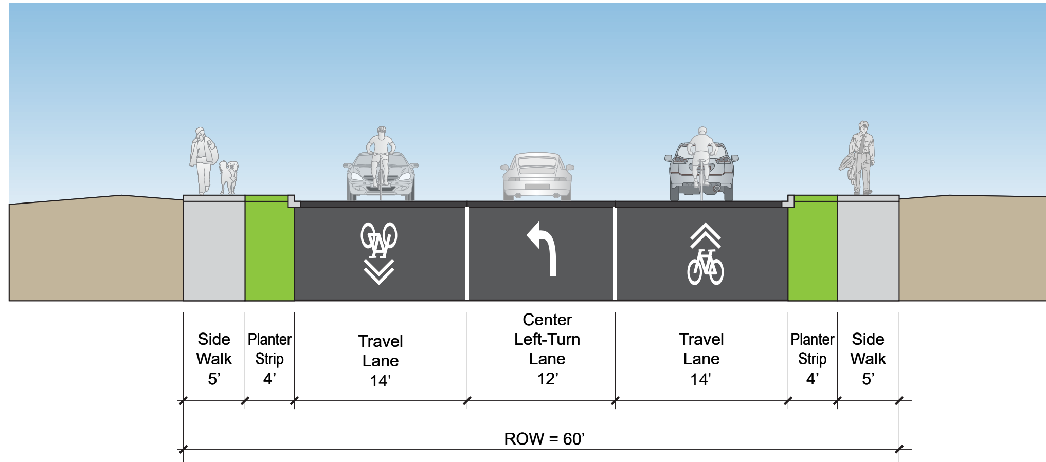
MAPLE ST. TYPICAL SECTION D-D
