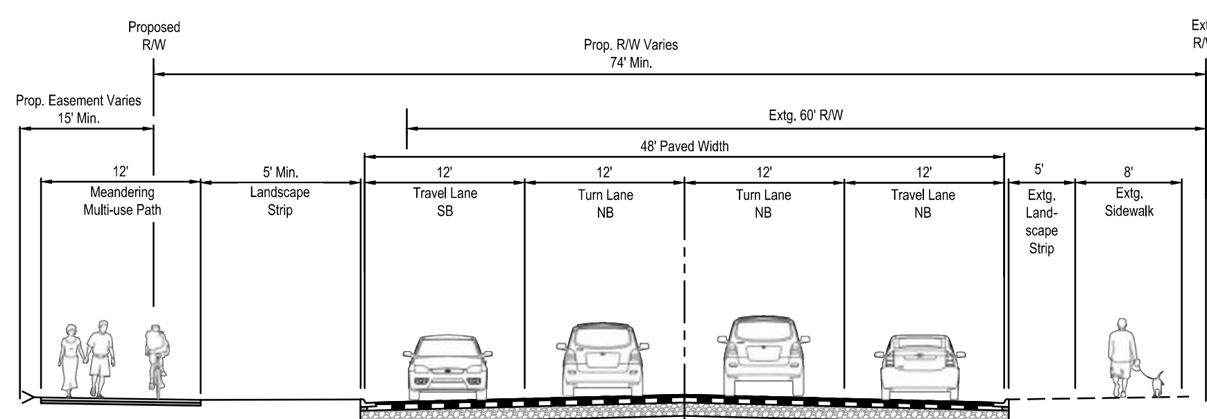
SECTION C-C
