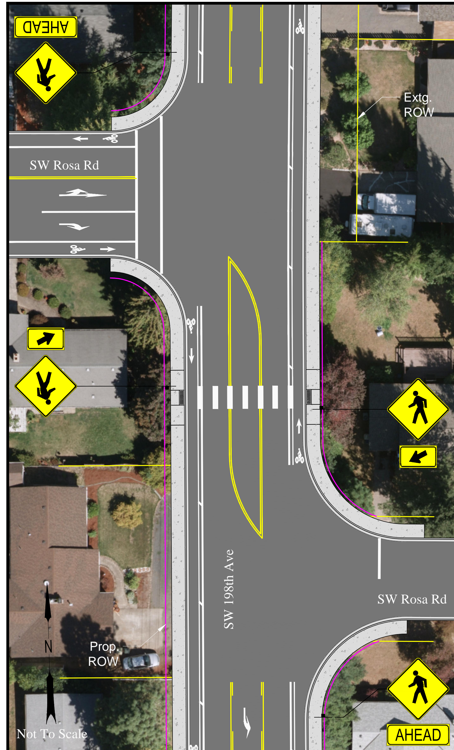
Alternative 1: Basic Mid-Block Crossing
