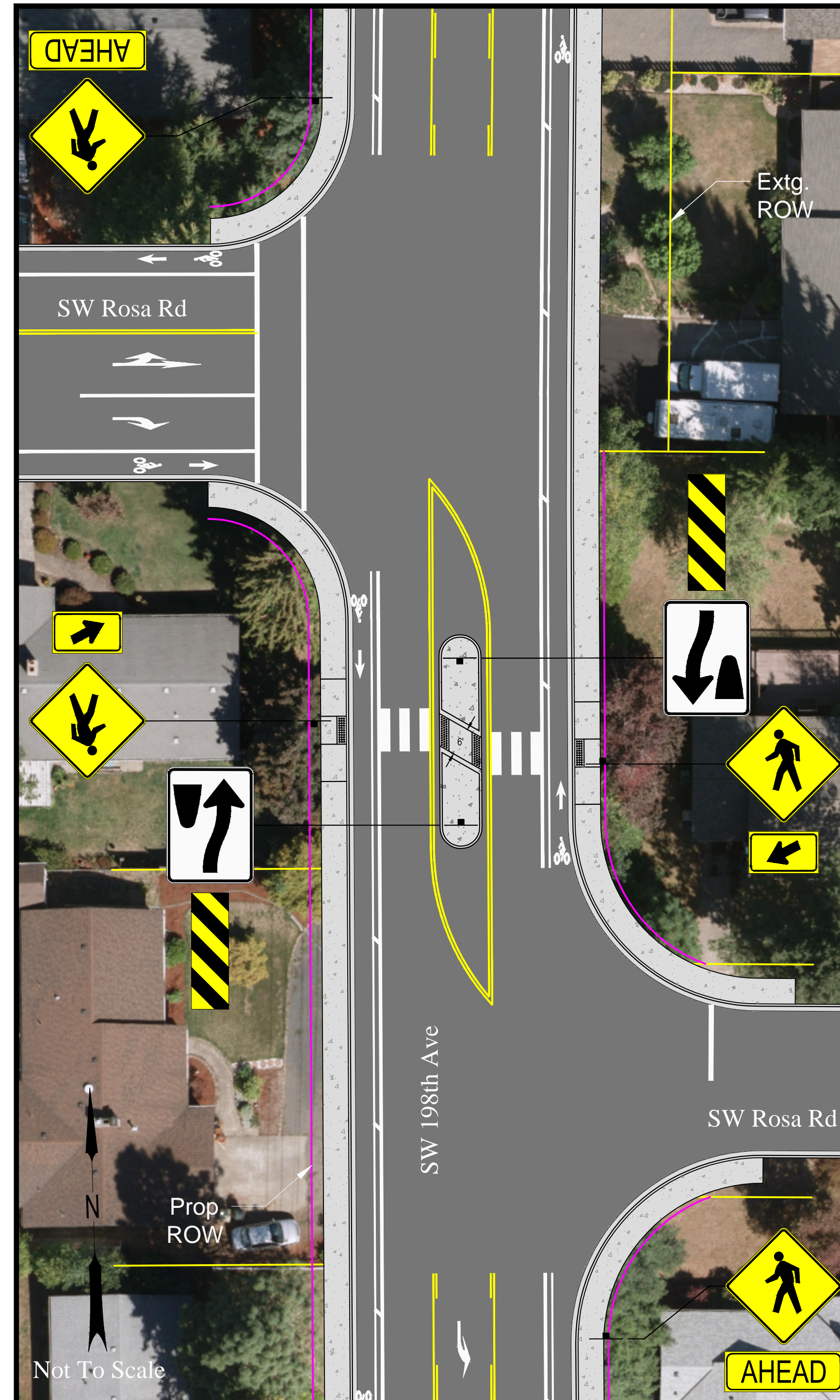
Alternative 2: Washington County Standard Mid-Block Crossing
