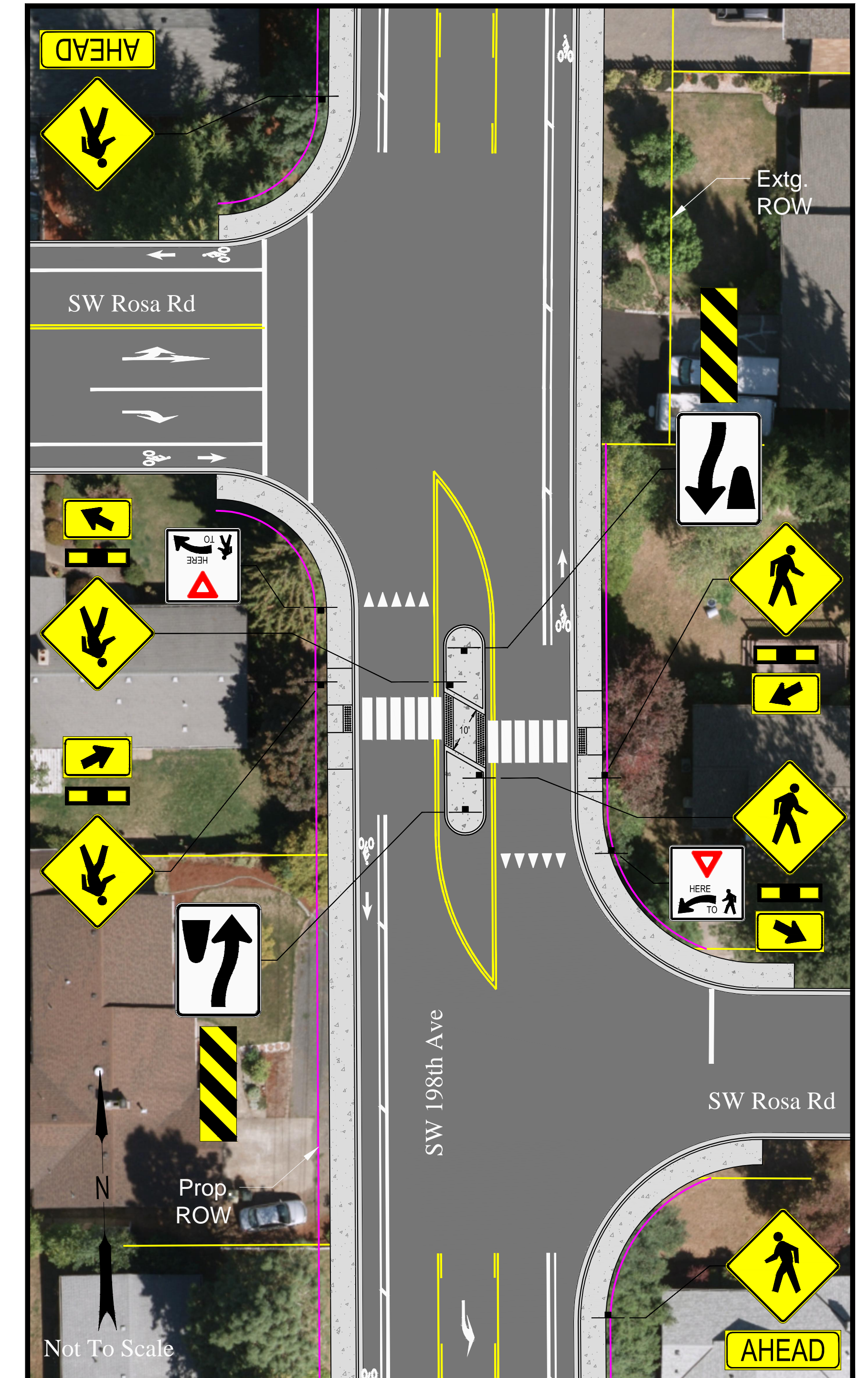
Alternative 3: Enhanced Mid-Block Crossing
