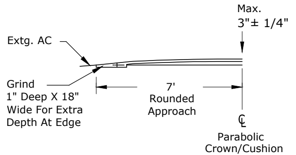
SECTION VIEW A - A Symetrical About CL N.T.S.
