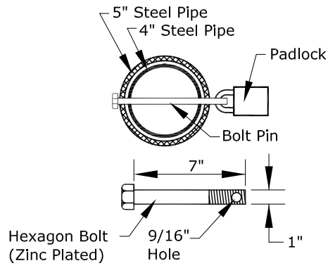
BOLT PIN DETAIL NTS
